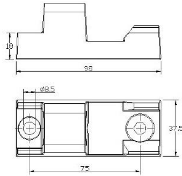
Yan Kapak Menteşesi Code DMK42 Side Board Hinge Code DMK42
