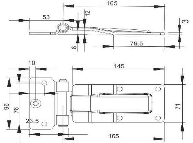
Paslanmaz/Stainless steel Code DMM25 Galvaniz/Galvanized steel Code DMM26
