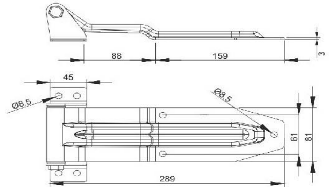
Paslanmaz/Stainless Steel Code DMM15 Galvaniz/Galvanized steel Code DMM16
