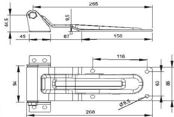
Paslanmaz/Stainless Steel Code DMM07 Galvaniz/Galvanized steel Code DMM08
