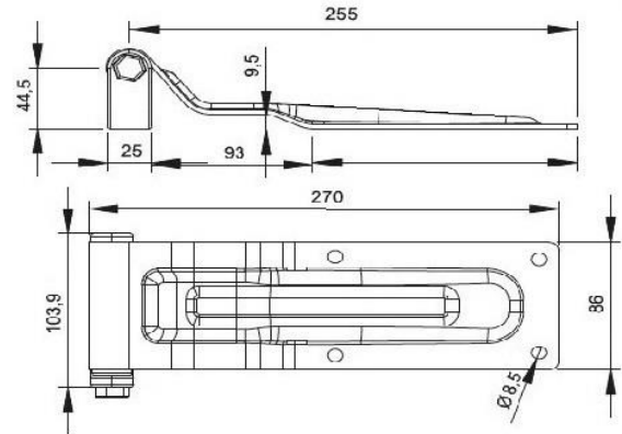
Paslanmaz/Stainless Steel Code DMM05 Galvaniz/Galvanized steel Code DMM06
