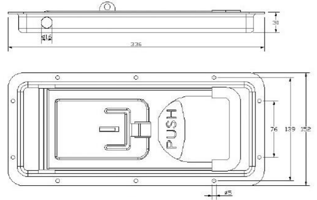
Paslanmaz/Stainless Steel Code DMK36 Galvaniz/Galvanized Steel Code DMK37
