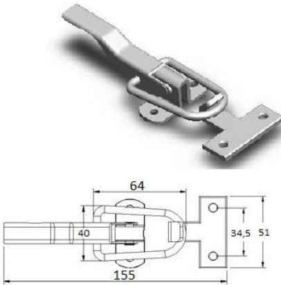
Mekanik kol Mechanical lever
