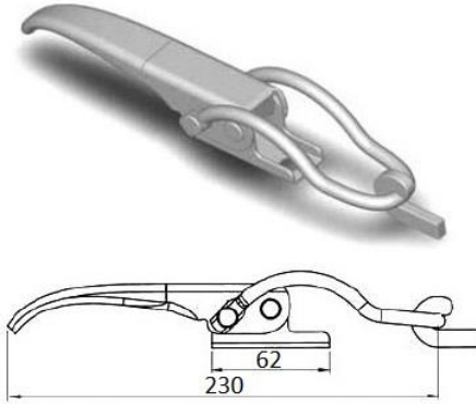
Mekanik kol Mechanical lever
