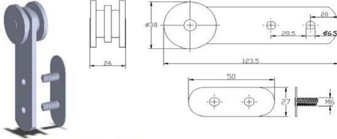
Makara Code DMR.08 Runner Code DMR.08
