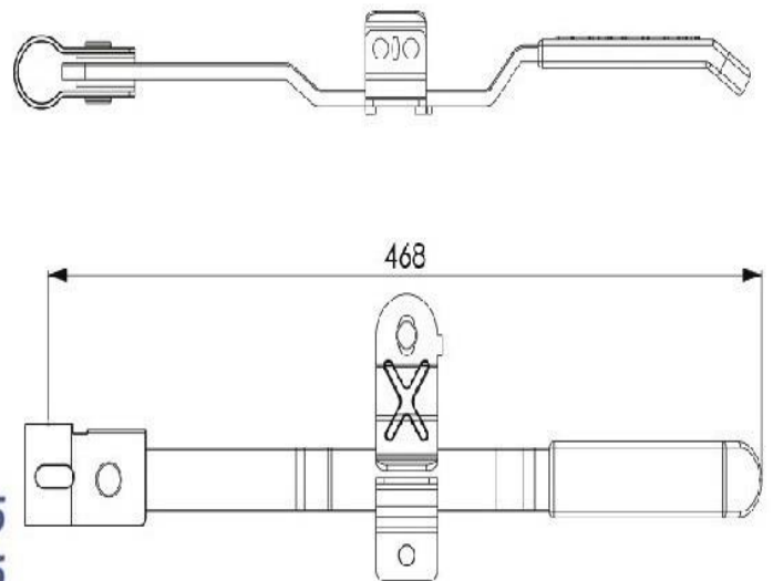
Paslanmaz/Stainless Steel Code DMK05 Galvaniz/Galvanized Steel Code DMK06
