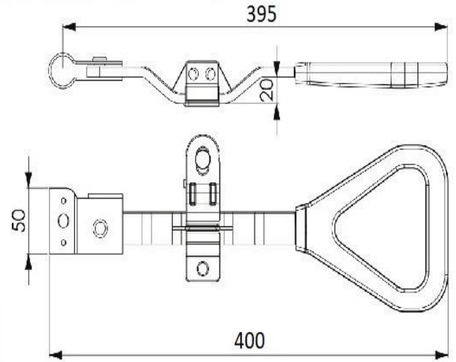
Paslanmaz/Stainless Steel Code DMK03 Galvaniz/Galvanized Steel Code DMK04
