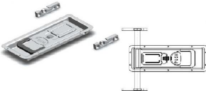
Paslanmaz/Stainless Steel Code DMK40 Galvaniz/Galvanized Steel Code DMK41
