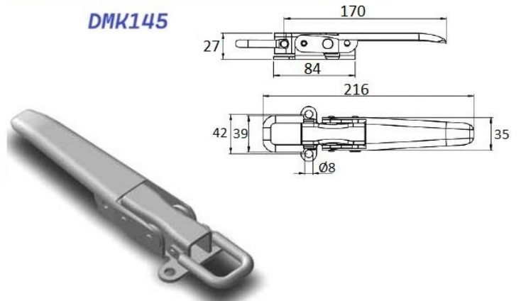
Mekanik kol Mechanical lever
