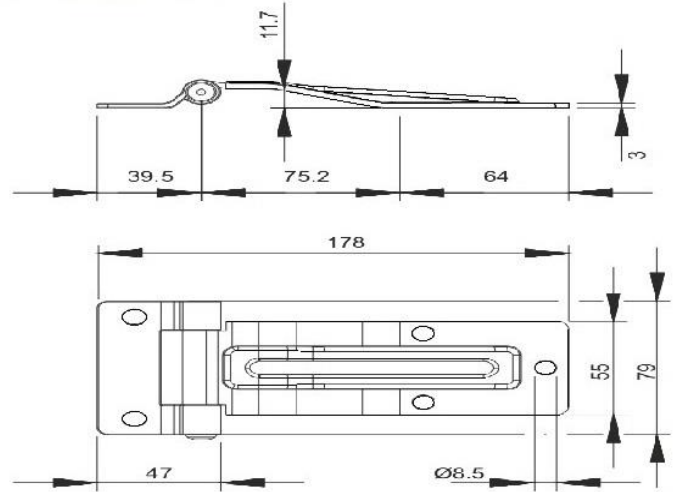
Paslanmaz/Stainless Steel Code DMM23 Galvaniz/Galvanized steel Code DMM24
