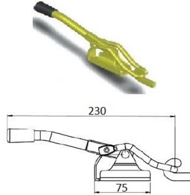
Hyundai mekanik kol Hyundai mechanical lever
