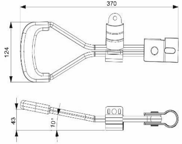
Paslanmaz/Stainless Steel Code DMK01 Galvaniz/Galvanized Steel Code DMK02
