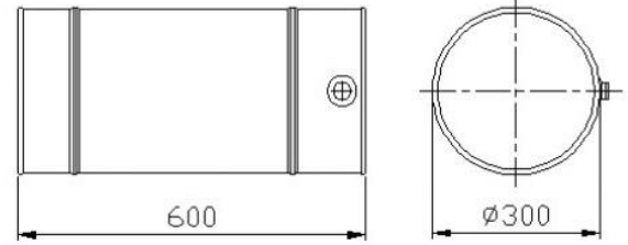
Su Deposu Paslanmaz / Water Tank Stainless Steel Code DMK57 Su Deposu Galvaniz / Water Tank Galvanized Steel Code DMK58
