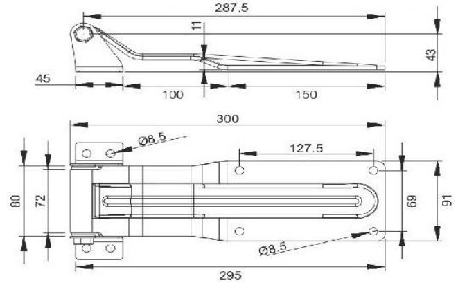
Paslanmaz/Stainless Steel Code DMM9 Galvaniz/Galvanized Steel Code DMM10
