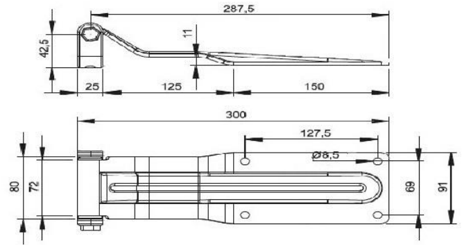
Paslanmaz/Stainless Steel Code DMM11 Galvaniz/Galvanized Steel Code DMM12
