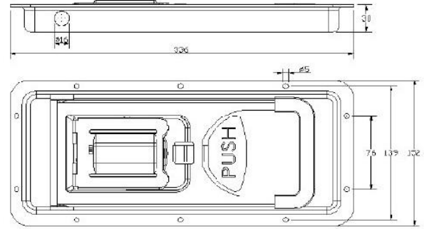
Paslanmaz/Stainless Steel Code DMK34 Galvaniz/Galvanized Steel Code DMK35
