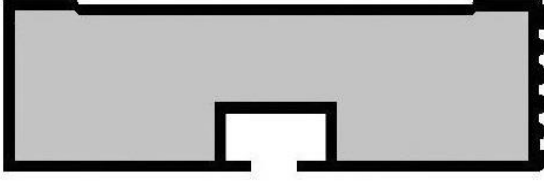
Pvc Bisikletlik Profili Code DMV.2859 Pvc Side Protecting Profile Code DMV.2859
