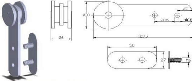
Makara Code DMR.08 Runner Code DMR.08
