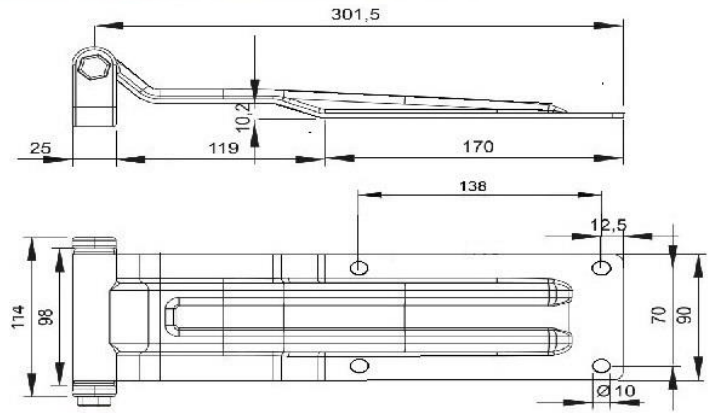
Paslanmaz/Stainless steel Code DMM03 Galvaniz/Galvanized steel Code DMM04
