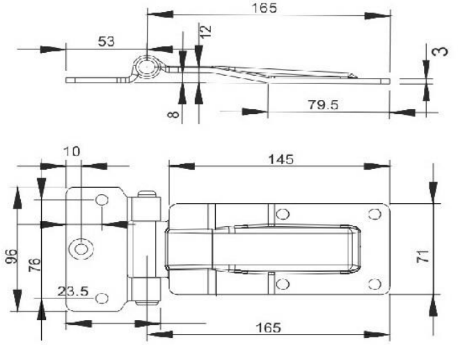
Paslanmaz/Stainless steel Code DMM27 Galvaniz/Galvanized steel Code DMM28
