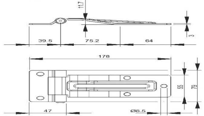
Paslanmaz/Stainless Steel Code DMM23 Galvaniz/Galvanized steel Code DMM24
