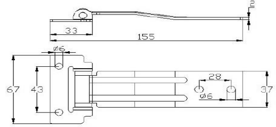
Paslanmaz/Stainless Steel Code DMM21 Galvaniz/Galvanized Steel Code DMM22
