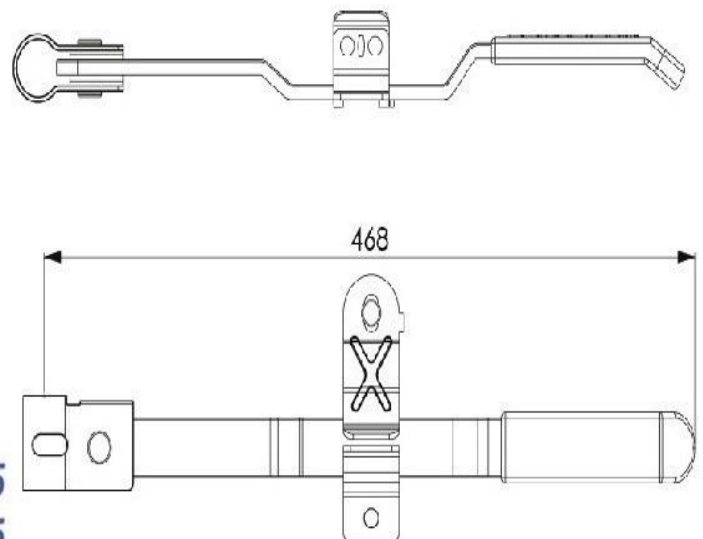
Paslanmaz/Stainless Steel Code DMK05 Galvaniz/Galvanized Steel Code DMK06
