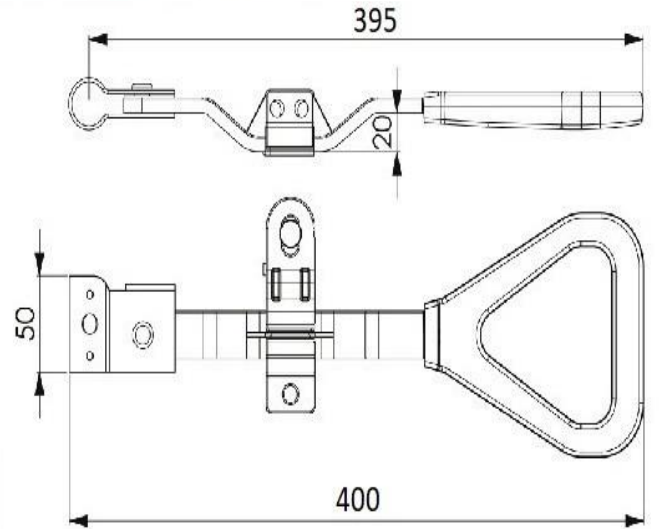
Paslanmaz/Stainless Steel Code DMK03 Galvaniz/Galvanized Steel Code DMK04
