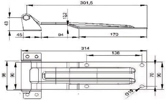
Paslanmaz/Stainless steel Code DMM01 Galvaniz/Galvanized Steel Code DMM02
