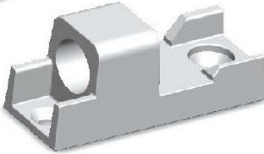
Yan Kapak Menteşesi Code DMK43 Side Board Hinge Code DMK43
