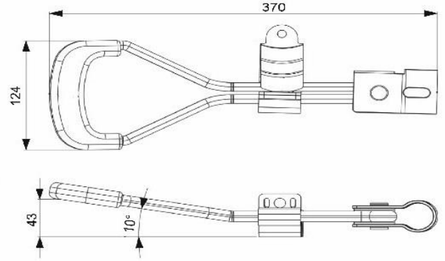
Paslanmaz/Stainless Steel Code DMK26 Galvaniz/Galvanized Steel Code DMK27
