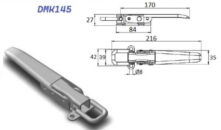
Mekanik kol Mechanical lever
