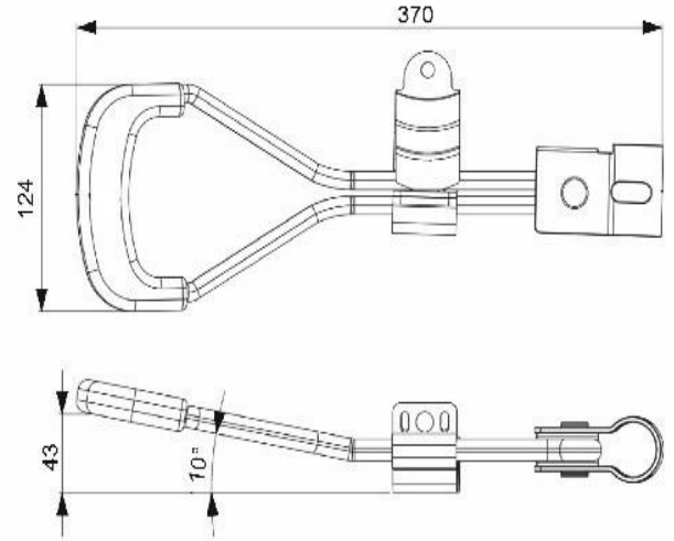
Paslanmaz/Stainless Steel Code DMK01 Galvaniz/Galvanized Steel Code DMK02
